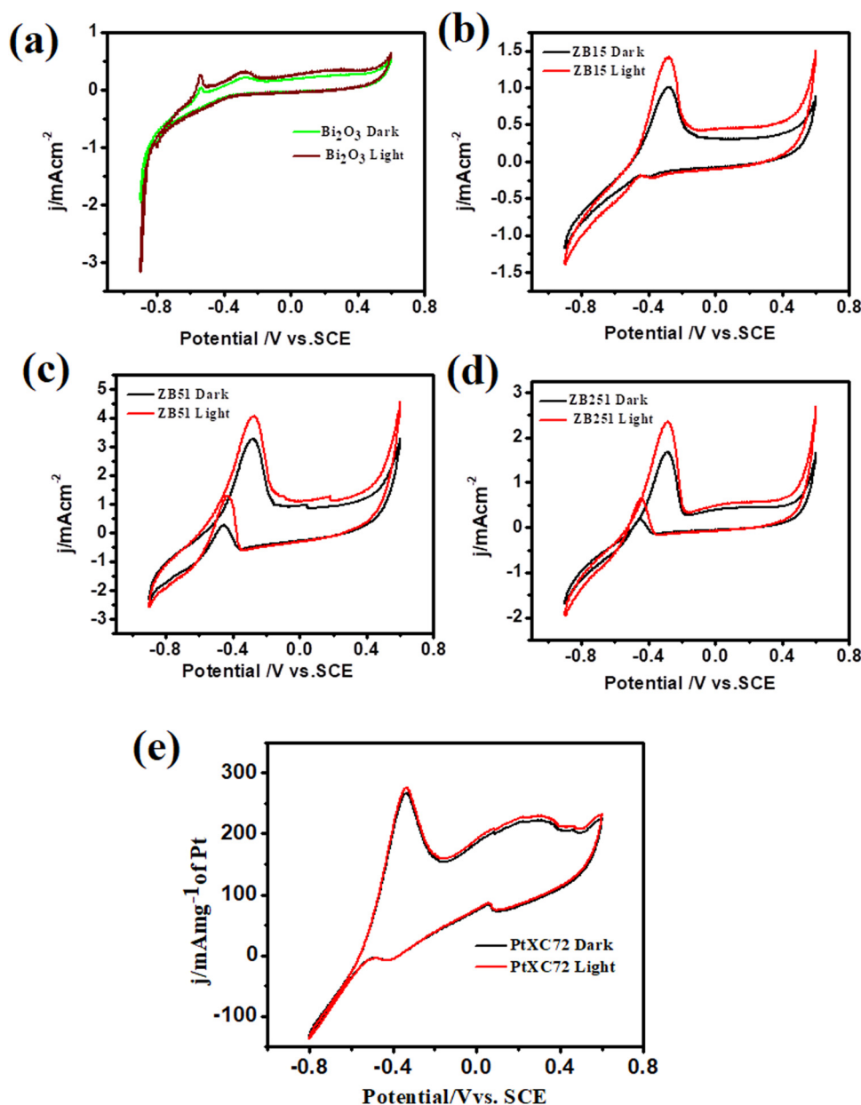
Fig. 6 Cyclic voltammograms of unplatined supports in 0.5 M MeOH + 1 M NaOH solution at 25 °C (a) Bi 2 O 3 (b) ZnO:Bi 2 O 3 (1:5) (c) ZnO:Bi 2 O 3 (5:1) (d) ZnO:Bi 2 O 3 (25:1) with and without irradiation.
