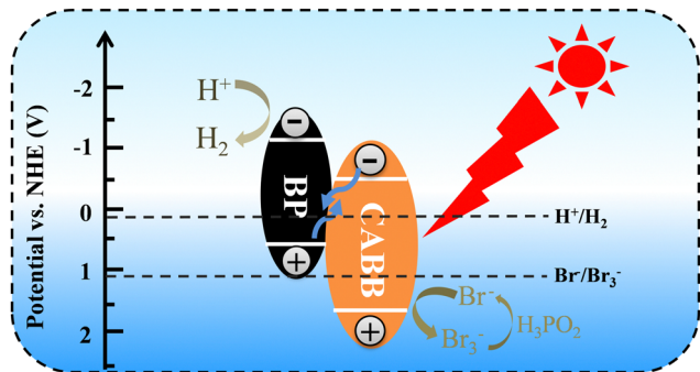
Fig. 6 Schematic illustration of the H 2 evolution of the BP/CABB composites.
