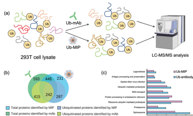
Fig. 6 (a) Schematic illustration of the identification and enrichment of ubiquitinated proteins in 293T cell lysates by Ub-mAb or Ub-MIP followed by LC-MS/MS analysis. (b) Total and overlaid proteins and ubiquitinated proteins identified by Ub-mAb and Ub-MIP. (c) Cluster analysis of the ubiquitinated proteins identified by Ub-mAb and Ub-MIP.
