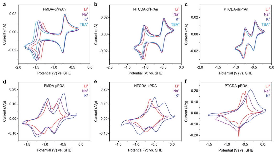
Fig. 2 Cyclic voltammograms at 50 \text{ mV s}^{-1} of solutions containing (a) PMDA- \text{di}^i\text{PrAn} , (b) NTCDA- \text{di}^i\text{PrAn} , and (c) PTCDA- \text{di}^i\text{PrAn} in DMF in the presence of \text{LiClO}_4 , \text{NaClO}_4 , \text{KClO}_4 , or TBA ^+ (0.1 M). Cyclic voltammograms at 0.25 \text{ mV s}^{-1} of (d) PMDA- \text{pPDA} , (e) NTCDA- \text{pPDA} , and (f) PTCDA- \text{pPDA} in metal (Li, Na, or K) half cells containing 1 : 1 EC : DEC (by vol) in the presence of \text{LiPF}_6 , \text{NaPF}_6 , or \text{KPF}_6 . The potential scales of the voltammograms were converted to potentials vs. SHE using tabulated values (see ESI ^\dagger for conversion values).
