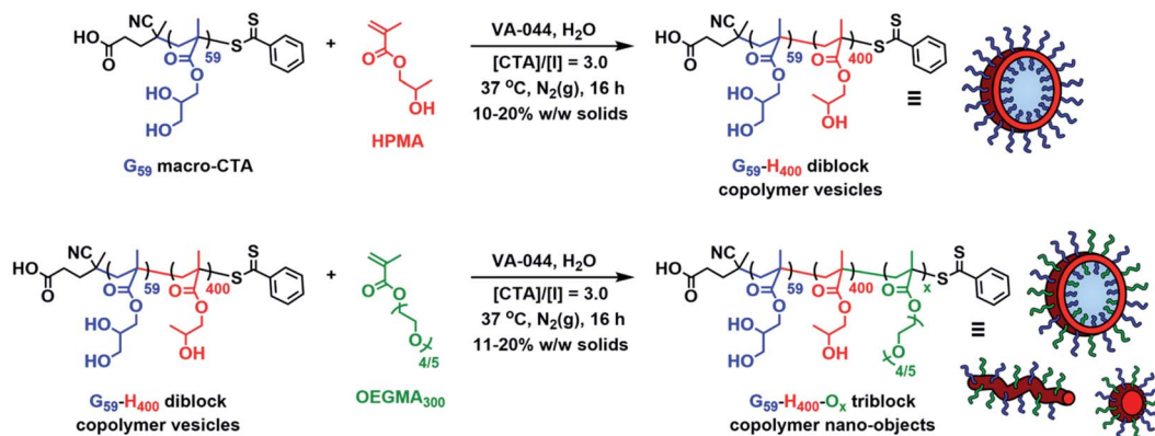
Scheme 1 Schematic illustration of the synthesis route employed for the preparation of poly(glycerol monomethacrylate) 59 -poly(2-hydroxypropyl methacrylate) 400 ( G_{59}\text{-H}_{400} ) diblock copolymer vesicles at 10–20% w/w solids via RAFT aqueous dispersion polymerization of HPMA using a G_{59} precursor, and their subsequent utilization as seed particles for the preparation of G_{59}\text{-H}_{400}\text{-O}_x triblock copolymer nano-objects at 11–20% w/w solids via RAFT-mediated aqueous polymerization-induced disassembly (PIDA).
