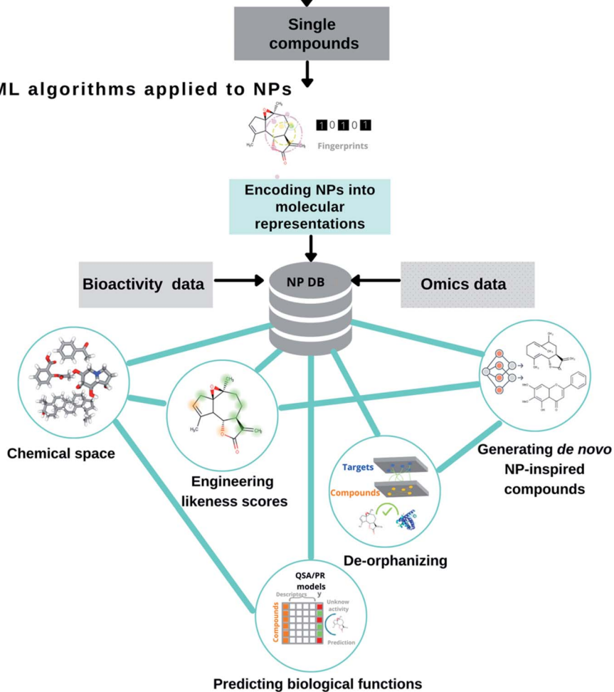
Fig. 1 Overview of ML/AI algorithms that are implemented across the different stages of the natural product drug discovery pipeline. The pipeline presents two sections: (1) computer-assisted discovery of NPs (data-mining into traditional medicines and peer-reviewed articles, genome mining & structural elucidation and dereplication) and (2) machine learning algorithms applied to NPs (encoding into molecular representations, molecular descriptors, likeness scores, chemical space, predicting biological functions, de-orphanizing and generating de novo NP-inspired compounds).
