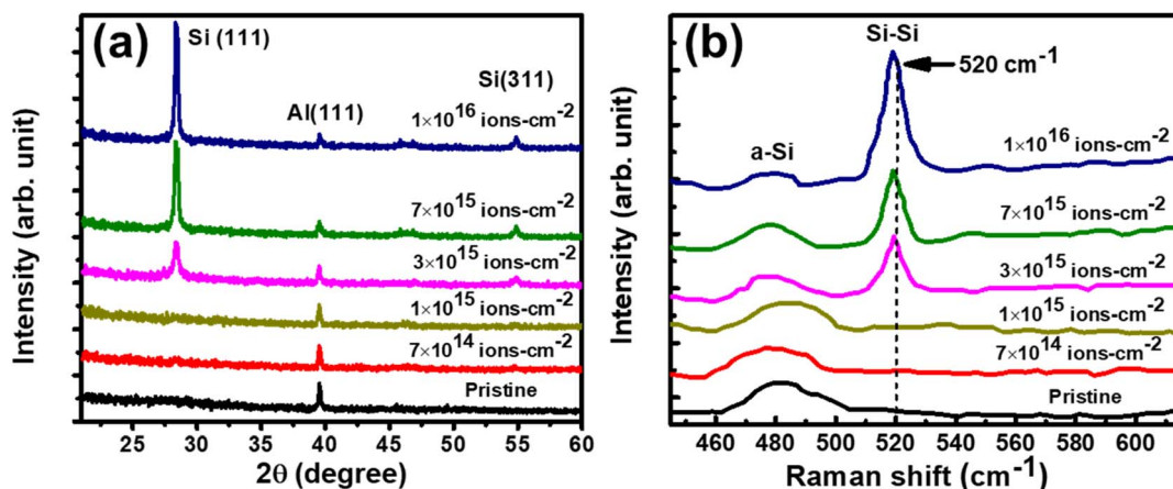
Fig. 10 (a) XRD pattern (b) Raman spectra of pristine sample and the samples irradiated with different ion fluence of 7 \times 10^{14} ions per \text{cm}^2 , 1 \times 10^{15} ions per \text{cm}^2 , 3 \times 10^{15} ions per \text{cm}^2 , 7 \times 10^{15} , and 1 \times 10^{16} ions per \text{cm}^2 . [Reproduced/adapted from Maity et al. , 161 J. Appl. Phys. , 2022, 132, 095303, with the permission from AIP Publishing.]
