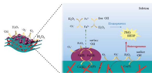
Fig. 12 Possible reaction mechanism of CoNWs@CoAl-LDHs/Fe 3 O 4 .
