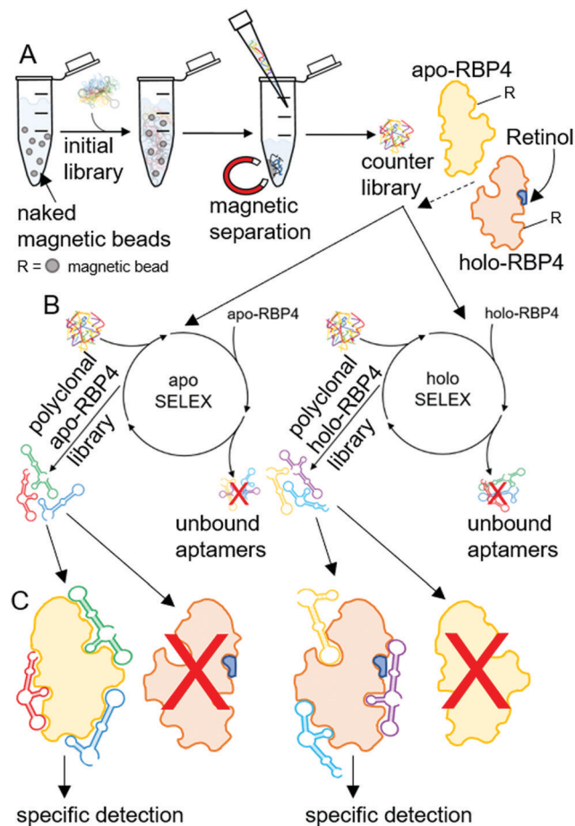
Scheme 2 SELEX based evolution of focused aptamer libraries for specific detection of apo- or holo-RBP4. (A) Initial counter selection by incubation of an initial aptamer library (~6 × 10 14 individual aptamers), containing 40 randomized nucleotides flanked by two primer binding sites, with naked Dynabeads ® M-280 tosyl-activated resulting in an aptamer 'counter library' with reduced amounts of aptamers with specificity against the naked beads. (B) Selection of specific polyclonal aptamer libraries by SELEX against apo- or holo-RBP4. Reduction of sequence diversity by incubating the counter selected aptamer library first with naked beads and subsequent with the target proteins (bound to Dynabeads ® M-280 tosyl-activated (indicated as 'R')) and aptamers exhibiting an adequate three-dimensional structure bind to the targets. The remaining unbound aptamers are subsequently removed, the bound aptamers are then eluted from the target proteins, amplified by ePCR and the undesired complementary strands are removed prior to the next SELEX round. (C) Specific target detection by binding of focused aptamer libraries. Exclusive binding of polyclonal apo-RBP4 aptamers to apo-RBP4 and of holo-RBP4 aptamers to holo-RBP4.
