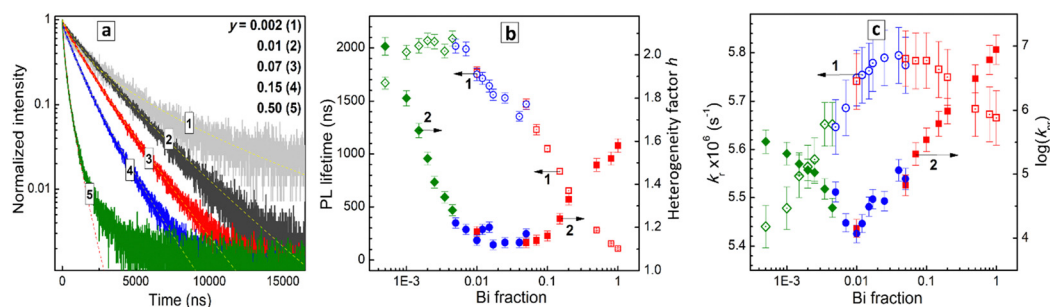
Fig. 7 (a) Kinetic curves of PL decay of CANBIC perovskites with Bi fraction \gamma = 0.002 (1), 0.01 (2), 0.07 (3), 0.15 (4), and 0.50 (5). Dashed lines represent the fitting of the experimental curves with a stretched exponential function. (b) PL lifetime (hollow scatters 1) and heterogeneity factor h (filled scatters 2) derived as functions of \gamma . (c) Rate constants of radiative recombination k_r (hollow scatters 1) and non-radiative recombination k_{nr} (filled scatters 2) as functions of \gamma . Shape of scatters indicates the range of Bi content variation: 0.1 (squares), 0.005–0.05 (circles), and 0.0005–0.005 (diamonds).
