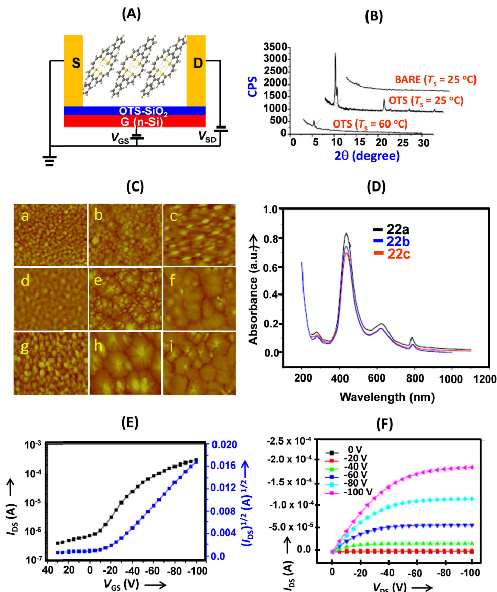
Fig. 6 (A) Schematic of the BGTC thin film OFET devices of 22a–c ; (B) X-ray diffraction patterns of the thin films of 22a deposited on \text{SiO}_2/\text{Si} (BARE) and OTS/ \text{SiO}_2/\text{Si} substrates at different temperatures; (C) AFM images ( 2 \times 2 \mu\text{m} ) of 50 nm thick films of 22a (a: BARE T_s = 25^\circ\text{C} ; b: OTS T_s = 25^\circ\text{C} ; c: OTS T_s = 60^\circ\text{C} ); 22b (d: BARE T_s = 25^\circ\text{C} ; e: OTS T_s = 25^\circ\text{C} ; f: OTS T_s = 60^\circ\text{C} ); 22c (g: BARE T_s = 25^\circ\text{C} ; h: OTS T_s = 25^\circ\text{C} ; i: OTS T_s = 60^\circ\text{C} ); (D) normalized UV-vis absorption spectra of thin films of 22a–c at room temperature; (E) transfer and (F) output characteristics of the thin film OFET devices (deposited on an OTS treated \text{SiO}_2/\text{Si} substrate ( T_s = 25^\circ\text{C} )) based on 22a . Reproduced with permission from ref. 13. Copyright 2011, The Royal Society of Chemistry.
