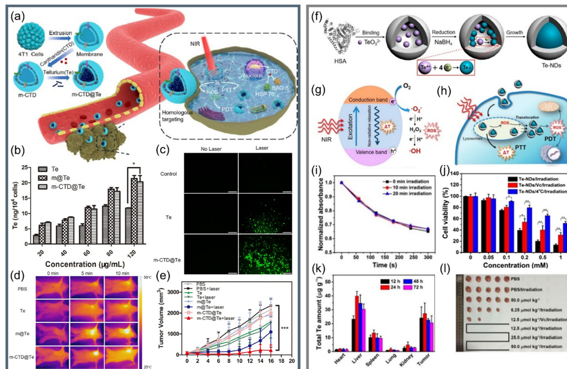
Fig. 9 (a) Schematic diagram of preparation of m-CTD@Te and synergistic anticancer applications. 121 (b) Content of Te in 4T1 cells after treatment with different groups by Te, m@Te, and m-CTD@Te. 121 (c) Exploring of the ability of Te and m-CTD@Te to generate ROS through DCFH-DA. 121 (d) Real-time thermography of mice after intravenous injection of Te, m@Te, m-CTD@Te, and PBS. 121 (e) Change curve of tumor volume during 16 days of treatment (Laser wavelength = 808 nm, 1.0 W cm -2 ). 121 Copyright 2020, Elsevier. (f) Schematic diagram of bifunctional Te-NDs synthesis with HSA as a nano reactor. 55 (g) and (h) show the photothermal effect and ROS generation of Te-NDs to realize PTT/PDT synergistic treatment, respectively. 55 (i) Relationship between the standard absorption of DPBF and Te-NDs irradiation time for 0 min, 10 min, and 20 min. 55 (j) A chart comparing the cell survival rate of the three groups. 55 (k) The total Te content of several main tissues after treated by Te-NDs for different periods of time. 55 (l) Pictures of mice tumors after treated for 30 days (Laser wavelength = 785 nm, 1.5 W cm -2 ). 55 Copyright 2017, American Chemical Society.
