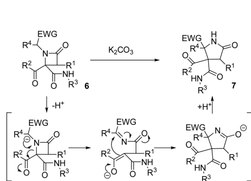
Scheme 2 Proposed mechanism for the anionic rearrangement from azetidinones 6 to pyrrolidinones 7 .
