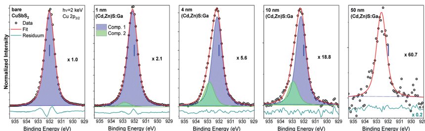
Fig. 3 Cu 2p_{3/2} HAXPES detail spectra recorded with 2 keV of the bare CuSbS 2 absorber (leftmost panel) and of the (Cd,Zn)S:Ga/CuSbS 2 samples with buffer thicknesses varying from 1 nm (panel second from left) to 50 nm (rightmost panel). Spectra have been normalized to the background at low BE. The background subtracted data is shown together with the fits and resulting residuals ( i.e. , [data – fit] – shown on different scale if required with scaling factor indicated as e.g. , \times 0.5 ). Additionally, the magnification factors are stated (as e.g. , \times 1.0 ) that were applied to show all spectra on the same intensity scale as that of the bare absorber. The vertical blue line indicates the BE position of the peak location in the spectrum of the absorber.
