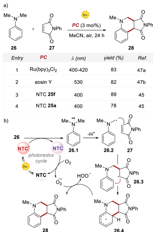
Scheme 14 (a) Povarov-type addition of N,N -dimethylaniline to phenylmaleimide. Comparison between the performance of \text{Ru}(\text{bpy})_3^{2+} and NTC 25f. (b) The reported mechanism for the Povarov-type addition of N,N -dimethylaniline to phenylmaleimide, depicted with NTCs as PCs.
