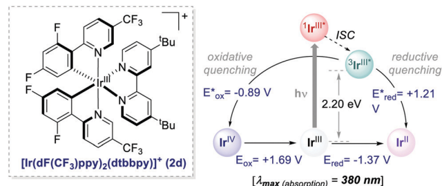
Scheme 23 Photophysical properties and redox potentials (in MeCN) of Ir(III) complex 2d (ref. 15).
