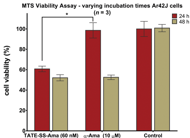
Fig. 8 Cell death kinetics of bioconjugate TATE-SS-Ama 6 and α-amanitin 1 evaluated on Ar42J cells following 24 and 48 hours of incubation (MTS, n = 3 ), data reported as mean \pm S.D.; * P < 0.01 ; control experiments are cells grown under the same conditions and treated with 0.5% DMSO (vehicle) culture media.
