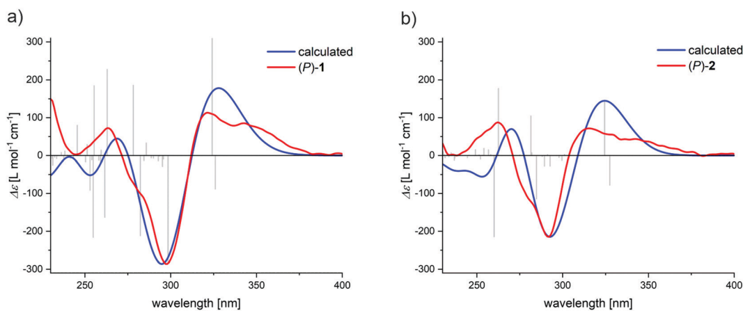
Fig. 8 Comparison of the experimental and calculated spectra for (P)-1 in (a) and (P)-2 in (b).
