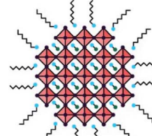
Nanocrystal (0D)
