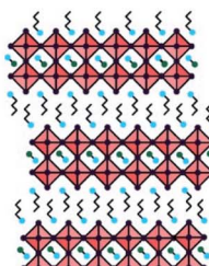
Layered (2D)
