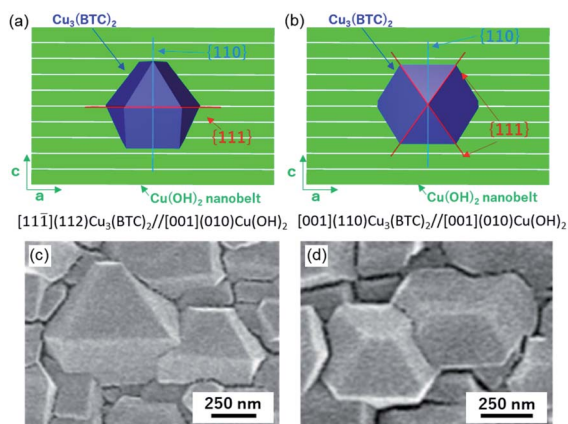
Fig. 2 Schematics and SEM images of the \text{Cu}_3(\text{BTC})_2 crystals epitaxially grown under [11\bar{1}](112)\text{Cu}_3(\text{BTC})_2//[\text{001}](010)\text{Cu}(\text{OH})_2 (a and c) and [001](110)\text{Cu}_3(\text{BTC})_2//[\text{001}](010)\text{Cu}(\text{OH})_2 (b and d) orientation relationships. The cuboctahedron-shaped crystals and green rectangles denote the \text{Cu}_3(\text{BTC})_2 crystals and \text{Cu}(\text{OH})_2 nanobelts, respectively. In the SEM images, the longitudinal direction ( a -axis) of the underlying \text{Cu}(\text{OH})_2 nanobelts is aligned horizontal to the images.
