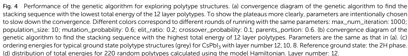
for different interlayer interactions, which only differ in sign. With the absolute values provided in Table 1, the impact of J_2 and K become pronounced because the absolute total contribution of interlayer interactions is at the 10 meV level, making the influence from the J_2 and K related terms non-negligible. Moreover, from the model Hamiltonian, why the ground state structures for CsPbBr 3 and CsPbI 3 polytypes prefer different stacking sequences can also be explained. By subtracting eqn (3) and (4), the energy difference between the 2H and 3C phases per layer is
