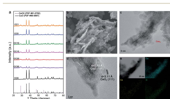
Fig. 1 (a) The XRD patterns of the CCX composites with various Ce contents. (b and c) The SEM and TEM images of the CC20 (the red circle represents the CeO_2 nanoparticles). (d) The HR-TEM image of the CC20. (e) The energy dispersive X-ray spectroscopy (EDS) maps of CC20.
