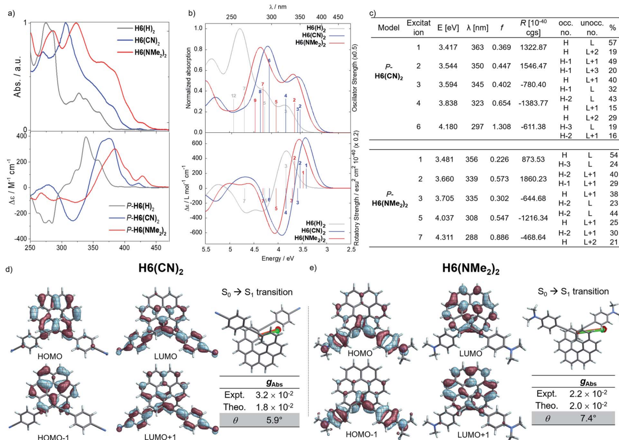
Fig. 5 (a) Top: UV-vis absorption (solid lines) and bottom: ECD spectra of H6(H) 2 (grey), H6(CN) 2 (blue) and H6(NMe) 2 (red) in dichloromethane at 298 K ([ ] ~10 -5 M); (b) calculated (Calc.) absorption (top) and ECD (bottom) of P-H6(H) 2 (grey), P-H6(CN) 2 (blue) and P-H6(NMe) 2 (red), selected transitions and oscillator and rotatory strengths indicated as 'stick bars'. (c) Details for the selected transitions and oscillator and rotatory strengths; (d and e) isosurfaces (±0.04 au) of the frontier molecular orbitals (MOs) with the corresponding electric (green) and magnetic (red) dipole moment vectors corresponding to excitation #2 (S 0 → S 1 transition), and the experimental (Expt.) and calculated (Theo.) absorption dissymmetry factor ( g ) and \theta angle (in degrees) for H6(CN) 2 and H6(NMe) 2 , respectively.
