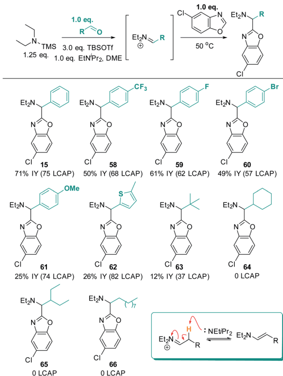
Scheme 16 Aldehyde scope. Conditions: azole (1.0 eq.), TBSOTf (0.416 mL, 1.813 mmol, 3.0 eq.), \text{TMS-NEt}_2 (1.25 eq.), PhCHO (1.0 equiv.), \text{EtN}^i\text{Pr}_2 (1.0 equiv.), \text{N}_2 , 50 °C, 18 h.
