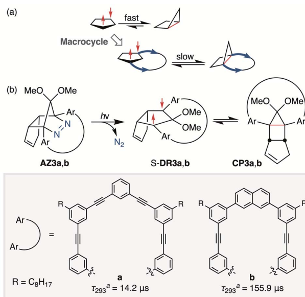
Scheme 2 (a) Stretch effect induced by the macrocycle. (b) Localised diradicaloids investigated in this study. a Lifetime values τ 293 were determined in benzene.
