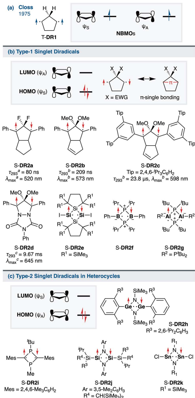
Scheme 1 (a) Pioneering work of Closs; (b) Type-1 and (c) Type-2 localised singlet diradicaloids in (hetero)cyclobutane and -pentane systems. The lifetime τ 293 and maximum absorption wavelength λ max were determined in a n -pentane, b benzene, or c toluene.
