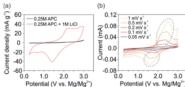
Fig. 2 Comparison of the electrochemical performance of 2 nd CV cycles of a V_2O_5 cathode at a scan rate of 0.1\text{ mV s}^{-1} (a) using the APC and APC + LiCl electrolyte and (b) CV scans at various scan rates ranging from 0.05 to 1\text{ mV s}^{-1} , using the APC + LiCl electrolyte.
