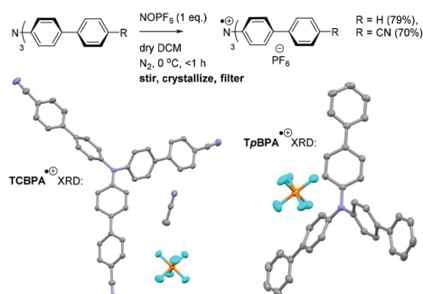
Fig. 7 Synthesis of \text{TpBPA}^{+\bullet} , \text{TCBPA}^{+\bullet} and their XRD crystal structures. Thermal ellipsoids are set at the 50% probability level. H atoms omitted for clarity; C atoms (grey), F atoms (cyan), N atoms (blue), P atoms (orange).
