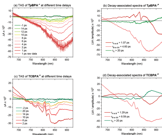
Fig. 8 Transient absorption and decay-associated spectra of \text{TPA}^{+\bullet} s.
