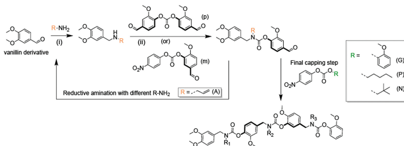
Fig. 1 General synthesis scheme for sequence-defined polyurethane macromers. (i) MeOH, NaBH 4 , room temperature, (ii) triethylamine, CH 3 CN, 50 °C., (A) – allyl, (G) – guaiacal, (P) – pentyl, (N) – neopentyl.
