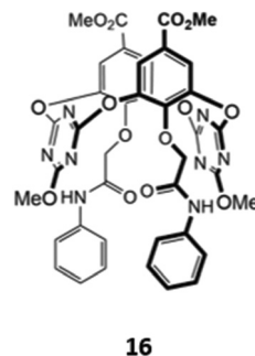
Fig. 5 Structure of an oxacalix[2]arene[2]triazine capable of sensing \text{H}_2\text{PO}_4^- ( K_a = 7.98 \times 10^3 \text{ M}^{-1} in \text{CH}_3\text{CN} ).
