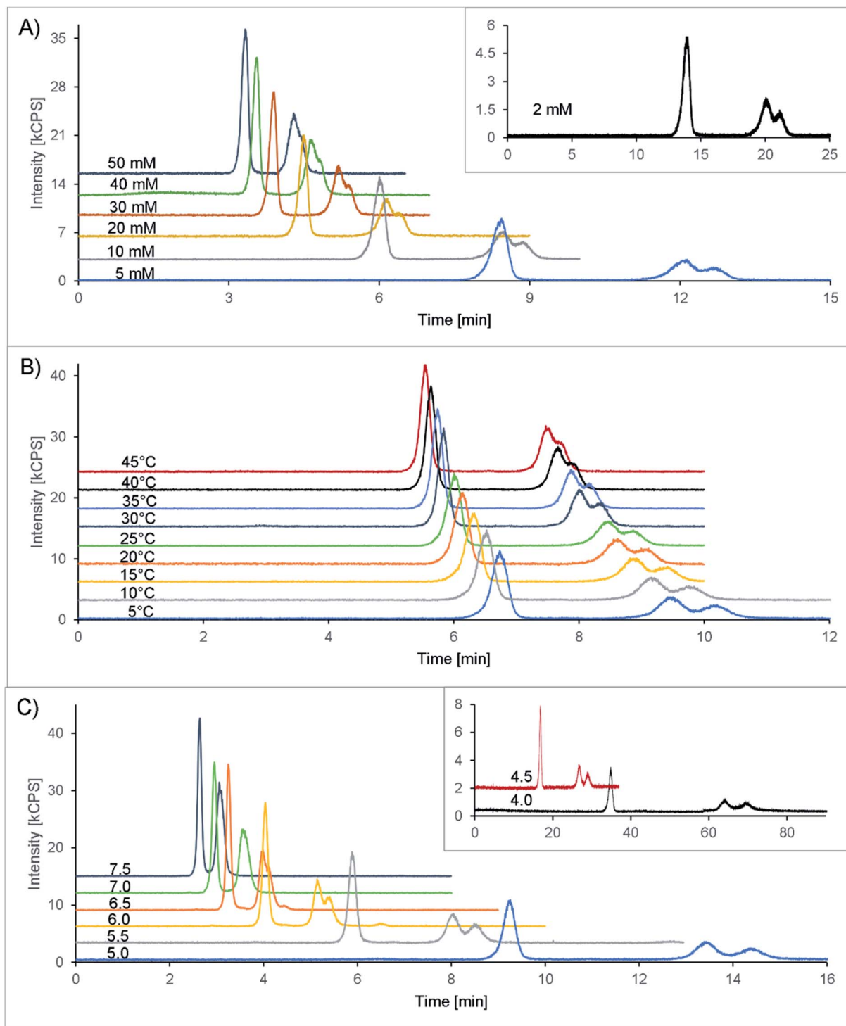
Fig. 3 HPLC-ICPMS chromatograms ( V at m/z 51) of amavadin (5 \mu\text{g V L}^{-1} , later-eluting double peak, corresponding to the two isomers) and vanadyl acetate (5 \mu\text{g V L}^{-1} , first peak) during method optimization. (A) Varying concentration of citric acid, at 25 °C and pH 5.3. The lowest concentration, 2 mM, is shown in the inset due to the much longer retention times. (B) Varying temperature, at 10 mM citric acid and pH 5.3. (C) Varying pH, at 10 mM citric acid and 10 °C. The chromatograms at pH 4.0 and 4.5 are shown in the inset due to the much longer retention times. Offsets of the y-axis in A, B and C: +3 kcps from the previous line. Exception: +1.5 kcps for pH 4.5 in the inset of C.
