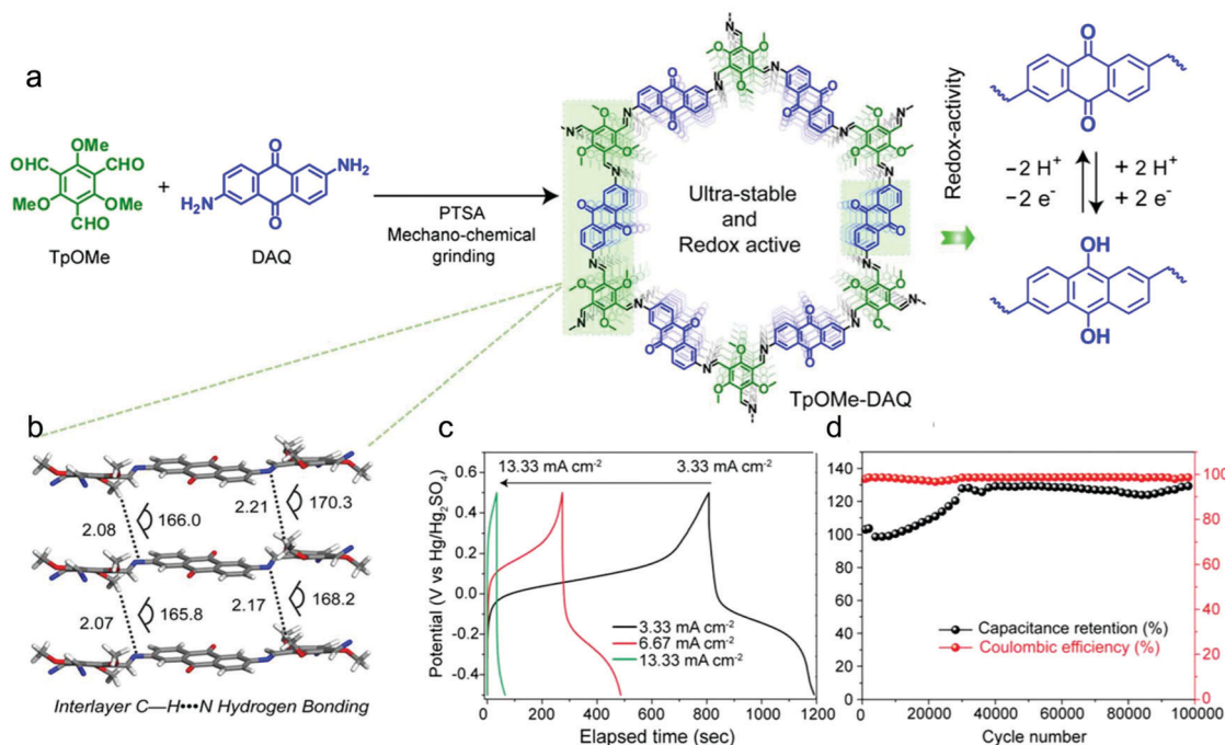
Fig. 16 (a) Schematic representation of the synthesis of TpOMe-DAQ, and the reversible transformation between quinone and hydroquinone; (b) structural illustration of the interlayer C-H...N-H-bonding in TpOMe-DAQ; (c) galvanostatic charge-discharge and (d) cycling stability performance (10 mA cm -2 ) of TpOMe-DAQ thin sheets. Reproduced from ref. 41 with permission from the American Chemical Society, copyright 2018.
