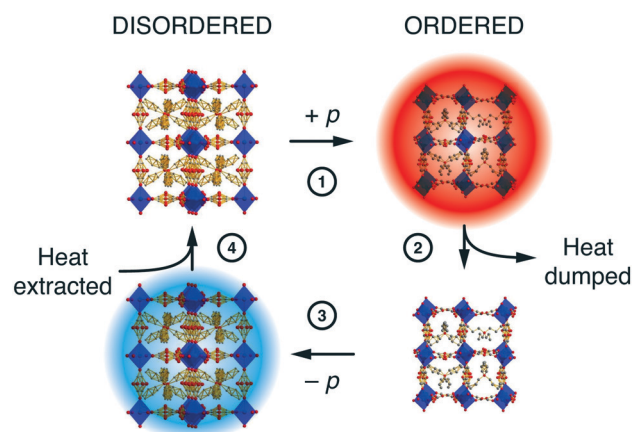
Fig. 5 A simple barocaloric cooling strategy that exploits the pressure-dependence of the order/disorder transition in [NPr_4][Mn(N(CN)_2)_3] . Starting at ambient conditions where the system is orientationally disordered (top left), ordering is induced by (1) application of pressure (note the change in unit cell dimensions is exaggerated here for effect). The loss of configurational entropy results in heating, and this excess heat (2) is dumped to the environment. (3) Removing the applied pressure forces the system to disorder; the concomitant increase in entropy now requires the system to cool. The cold solid (4) extracts heat from its environment. 74,75 Adapted from ref. 74 with permission from Springer Nature.
