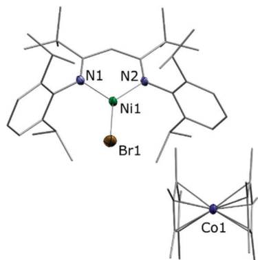
Fig. 1 Molecular structure of [\text{L}^{\text{tBu}}\text{NiBr}][\text{Cp}^*\text{Co}] \cdot 3\text{C}_7\text{H}_8 . Hydrogen atoms are omitted for clarity. Selected bond lengths/Å and angles/ ^\circ : N1–Ni1 1.895(4), N2–Ni1 1.904(4), Ni1–Br1 2.3447(8), N2–Ni1–N1 98.67(16), N1–Ni1–Br1 134.78(12), N2–Ni1–Br1 126.53(12), ave. Co–C CP = 2.051(6), ave. Co–C pcent = 1.655(3).
