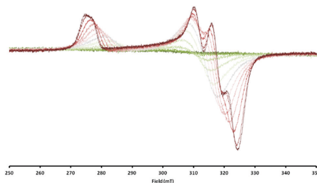
Fig. 3 Overlaid EPR spectra of [\text{L}^{\text{tBu}}\text{NiBr}][\text{Cp}_2\text{Co}] in toluene measured between 20 °C (dark green, silent) and -95 °C (dark red, up to ~60%).
