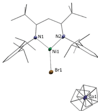
Fig. 2 Molecular structure of [\text{L}^{\text{tBu}}\text{NiBr}][\text{Cp}_2\text{Co}] . Hydrogen atoms are omitted for clarity. Selected bond lengths/Å and angles/ ^\circ : N1–Ni1 1.898(4), N2–Ni1 1.891(4), Ni1–Br1 2.3443(8), N2–Ni1–N1 99.18(17), N1–Ni1–Br1 130.55(12), N2–Ni1–Br1 130.26(12), ave. Co–C CP = 2.026(5), ave. Co–C pcent = 1.629(3).
