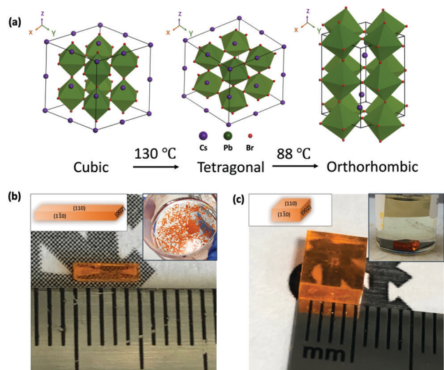
Fig. 1 (a) CsPbBr 3 structure at different temperature. The transition from cubic to tetragonal happens at 130 °C, and transition from tetragonal to orthorhombic happens at 88 °C. (b) Bar shape CsPbBr 3 single crystal grown without CB. The left inset indicates the miller indices of each surface, and the right inset is the photograph of crystals in solution. (c) Cuboid shape CsPbBr 3 single crystal grown with CB. The left inset indicates the miller indices of each surface, the right inset is the photograph of crystals in solution, and the bottom of the vial is a Si-wafer to make a flat bottom.
