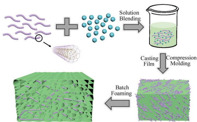
Fig. 1 Schematic diagram for the fabrication process of the PVDF/MWCNT nanocomposite foams.
