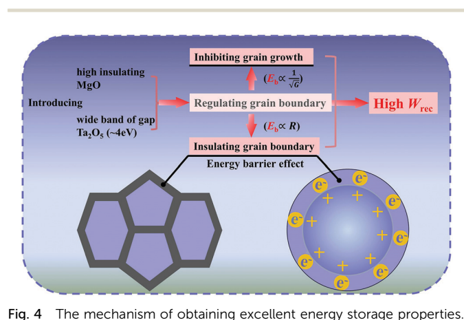
Fig. 4 The mechanism of obtaining excellent energy storage properties.
