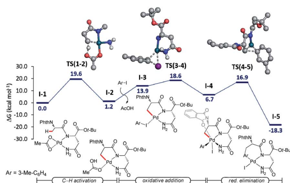
Fig. 2 Computed relative Gibbs free energies ( \Delta G_{403.15} ) in \text{kcal mol}^{-1} for palladium(II)-catalyzed \text{C}(\text{sp}^3)\text{--H} arylation at the PW6B95-D4/def-TZVP+SMD(DCE)//PBE0-D3BJ/def2-SVP level of theory. Non-relevant hydrogen atoms on the transition state structures were omitted for clarity.
