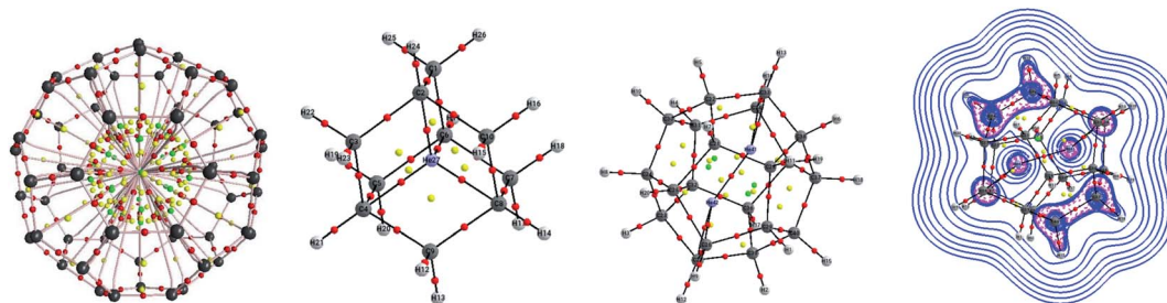
Fig. 6 Molecular graph of Ne@C 60 , He@adam, and He 2 @C 20 H 20 . The plot of the Laplacian of electron density for the latter complex is also given. Spheres in red, yellow, and green are the bond, ring, and cage critical points.
