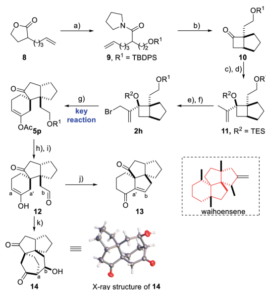
Scheme 3 Synthetic utility of the tetracyclic skeleton of waihoensene. Reagents and conditions: (a) pyrrolidine, Et 3 N, neat, 85 °C, then TBDPSCI, imidazole, CH 2 Cl 2 , 0 °C (98%); (b) Tf 2 O, 2,6-di- tert -butyl-4-methylpyridine, DCE, reflux, then CCl 4 /H 2 O reflux (54%); (c) 2-bromopropene, t -BuLi, THF, −78 °C (85% brsm); (d) TESOTf, 2,6-lutidine, CH 2 Cl 2 , 0 °C (94%); (e) SeO 2 , TBHP, CH 2 Cl 2 , 0 °C – rt (73% brsm); (f) CBr 4 , PPh 3 , imidazole, CH 2 Cl 2 , rt (90%); (g) prop-2-yn-1-yl acetate, CuOAc, Cs 2 CO 3 , DCE, 70 °C, then AuCl 3 , PTS, HFB (hexafluorobenzene), rt (40%, dr = 3.2 : 1); (h) TBAF, THF, 0 °C (93%); (i) IBX, EtOAc, reflux (91%); (j) K 2 CO 3 , MeOH/H 2 O = 100 : 1, 0 °C – rt (64%); (k) HCl, THF, rt (89%). TBDPSCI = tert -butyl diphenylchlorosilane, DCE = 1,2-dichloroethane, TESOTf = triethylsilyl tri-fluoromethanesulphonate, IBX = 2-iodoxybenzoic acid.
