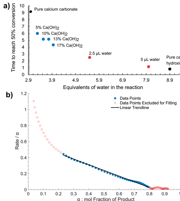
Fig. 5 (a) The reaction rate measured as the time required to reach 50% conversion as a function of the total equivalents (relative to calcium) of water present and/or generated in the system. (b) Reaction rate (d\alpha/dt)/\alpha vs. \alpha , where \alpha is the mol fraction of 1 as determined by in situ Raman spectroscopy for the synthesis using \text{CaCO}_3 reactant. Linear behaviour is observed between \alpha = 0.2 and 0.8 , consistent with autocatalysis due to a reaction product. Fitting parameters are reported in the ESI.†
