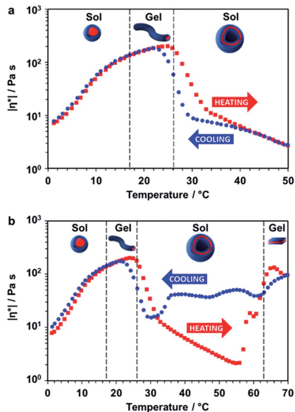
Fig. 3 Thermally-induced change in complex viscosity for an aqueous dispersion of linear diblock copolymer nano-objects. Temperature-dependent rheological studies for a 20% w/w aqueous dispersion of \text{PDMAC}_{56}\text{-P(HBA-stat-DAAM)}_{264} nano-objects at an applied strain of 1.0% and an angular frequency of 1.0 \text{rad s}^{-1} . The dispersion was equilibrated at 1 °C for 15 min prior to heating. The black dashed lines indicate the sol-gel transitions observed on heating as determined from the G' and G'' values (Fig. S3, ESI†). (a) Complex viscosity ( |\eta^*| ) vs. temperature data obtained for a thermal cycle from 1 °C to 50 °C to 1 °C at a heating/cooling rate of 1 °C \text{min}^{-1} [■ heating curve, ● cooling curve]. (b) Complex viscosity vs. temperature data for a thermal cycle over an expanded temperature range of 1 °C to 70 °C to 1 °C at a heating/cooling rate of 1 °C \text{min}^{-1} [■ heating curve, ● cooling curve].
