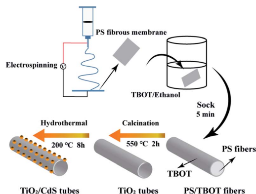
Fig. 1 An illustration of the formation mechanism of the TiO 2 /CdS nanotubes.
