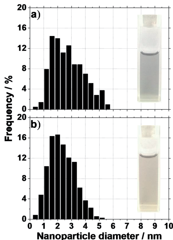
Fig. 2 Size distribution of Pt NPs obtained after 2 hours UV irradiation of a solution of 2 mM \text{H}_2\text{PtCl}_6 without NaOH in (a) methanol and (b) ethanol. Images of the solution after UV-irradiation are also displayed (volume is 3 mL).
