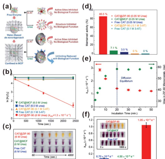
Fig. 9 (a) De novo approach and structural confinement of CAT@ZIF-90. (b and c) Kinetic measurements of H 2 O 2 degradation of free CAT, CAT@MCF, and CAT@ZIF-90 incubated with urea and 3-AT. All assays are performed in Tris buffer (pH 7.5, 50 mM). (d) Maintained activity of free CAT, CAT@MCF and CAT@ZIF-90 incubated in 0.05 M urea, and CAT@ZIF-90 incubated in 0.1 M 3-AT. (e) Amounts of urea diffused into ZIF-90 microcrystals (green) and K_{obs} of CAT@ZIF-90 (red) after incubation in 6 M urea for various periods of time. (f) Apparent rate constants after treatment at 80 °C for 3 min (inset shows photographs of time-dependent FOX assay). Reproduced with permission. 29 Copyright©2017 American Chemistry Society.
