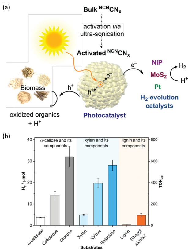
Fig. 6 (a) Schematic photo-reforming of lignocellulose using \text{NCN/CNx} and proton reduction co-catalysts. (b) Photocatalytic \text{H}_2 production from purified lignocellulose components catalyzed by activated \text{NCN/CNx} and NiP under AM1.5G light irradiation for one day at 25^\circ\text{C} . Reprinted from ref. 48 with permission of American Chemical Society, copyright 2018.
