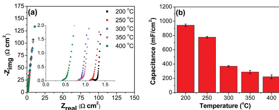
Fig. 10 (a) Nyquist plots for \text{RuO}_2 -CNF electrodes prepared at different temperatures (inset: the zoomed-in high-frequency region). The spectra were recorded at cell potential of 0 V (b) capacitance values obtained from EIS measurements for electrodes prepared at different temperatures.
