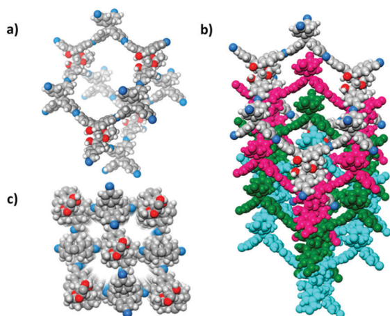
Fig. 11 Structural representation of CCOF 5. (a) Adamantine-like cage in the diamond net. (b) Structure viewed along the a -axis showing 4-fold interpenetration of a diamond net. (c) Two kinds of 1D channels long the c -axis. C gray; N blue; H white; O red. Adapted from ref. 86 with permission from the American Chemical Society, copyright 2018.
