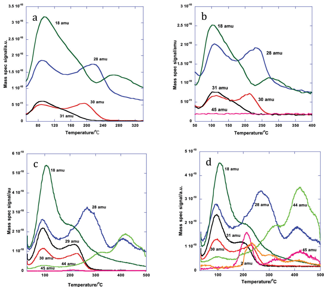
Fig. 3 Desorption products during TPD from the doped HSA Fe 2 O 3 samples, coated with 3 ML equivalent of MoO x : (a) 5% Al doped, (b) 10%, (c) 15% and (d) 20%.
