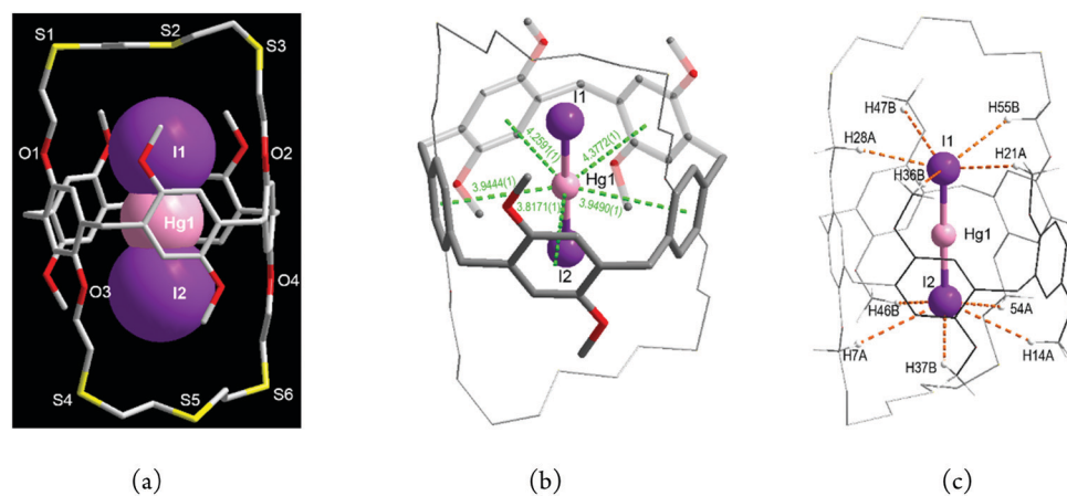
Fig. 4 The contact ion-triplet complex with mercury(II) iodide [(\text{I}-\text{Hg}-\text{I})@L] ( 3 ): (a) general view showing an ( \text{I}^--\text{Hg}^{2+}-\text{I}^- ) entity (space-filling) in the central cavity, (b) a pentagonal bipyramidal geometry with five \text{Hg}^{2+}\cdots\pi interactions (green dashed lines) and an \text{I}-\text{Hg}-\text{I} axis and (c) a mercury-shared double pentagonal pyramidal geometry with five \text{C}-\text{H}\cdots\text{I}^- H-bonds (orange dashed lines) and \text{I}-\text{Hg}-\text{I} axis (only H-bonded H atoms are shown).
