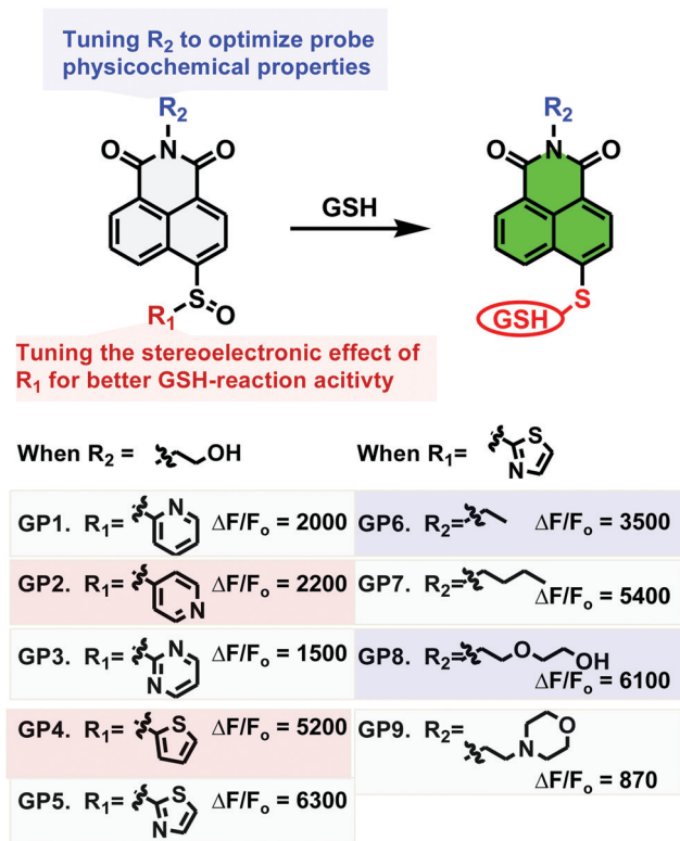
Fig. 1 Tuning the stereoelectronic effect and physicochemical property of sulfanyl naphthalimides for sensitive GSH probes. Designed probes (5 \mu M) were tested for their fluorogenic response towards GSH (2 mM) in PBS (10 mM, pH 7.4), and the degree of fluorescence increase ( \Delta F/F_0 ) was compared.
