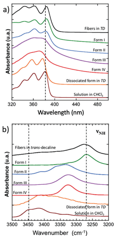
Fig. 5 (a) UV-vis spectra of the four polymorphs of NDI2 and in solution in chloroform and in trans -decaline (TD). The dissociated form in TD is obtained at T = 120^\circ\text{C} . (b) FTIR spectra (thin films) of the four polymorphs of NDI2, the melt and the solutions in TD. In both plots, the successive spectra were offset along the ordinate axis for clarity.
